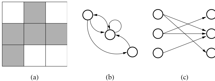
Figure 11. Two ways of transforming a given adjacency matrix (left) into ANNs. First, the graph is directly interpreted with recurrent neural connections (middle). Second, the adjacency matrix as a description of a feed-forward network (right).
